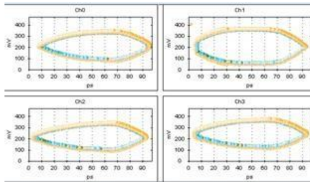
Figure 26: 4 Channels Eye Contour
