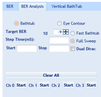
Figure 22: Bathtub Configuration
