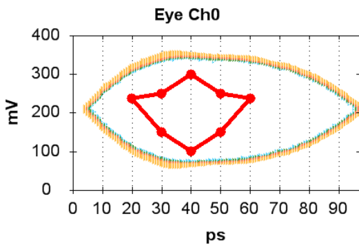
Figure 27: Eye Mask
