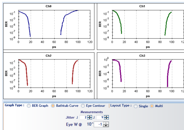
Figure 21: Bathtub Graph
