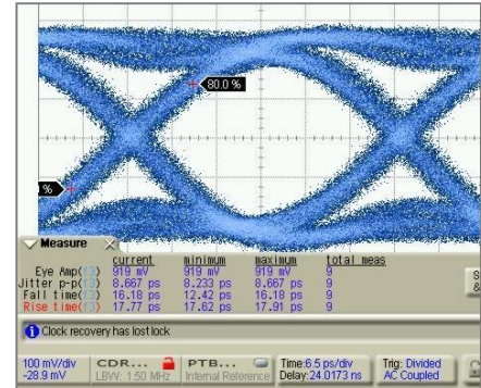
Figure 1: Eye Display
