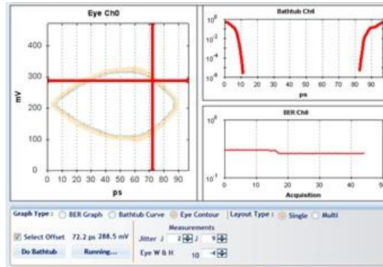
Figure 25: Single Channel Eye Contour
