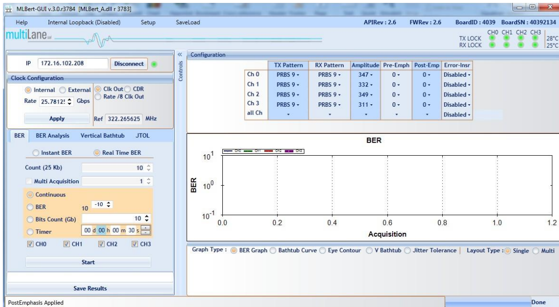
Figure 2: ML4039BERT GUI
